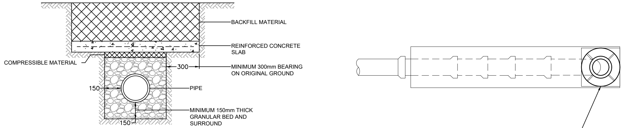
FIGURE B 27 PROTECTION OF PIPE LAID AT SHALLOW DEPTHS SCALE 1:20
