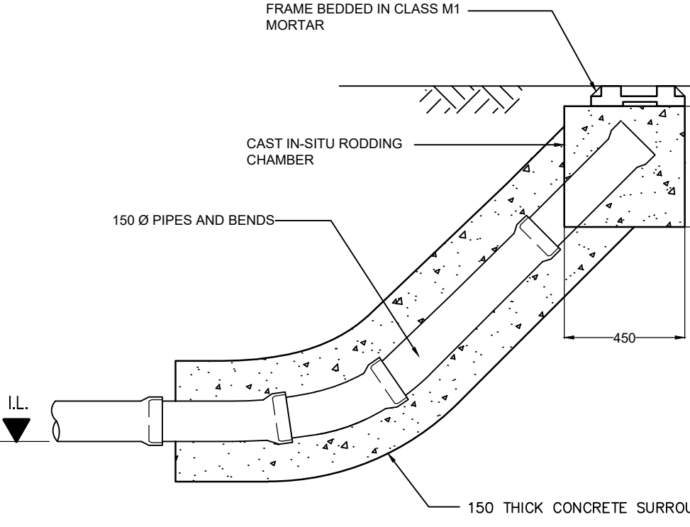
TYPICAL RODDING EYE PLAN & SECTION NTS
