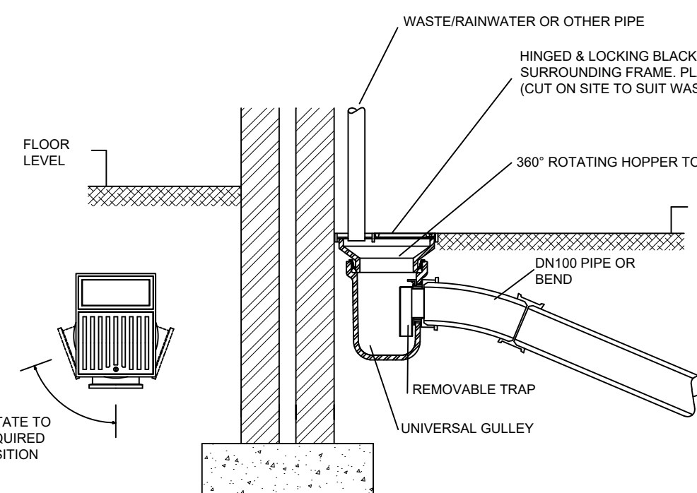
WASTE / RAINWATER OR OTHER PIPE CONNECTION TO UNIVERSAL GULLY NTS
