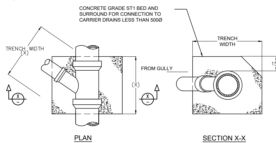
TYPICAL GULLY CONNECTION DETAILS NTS
