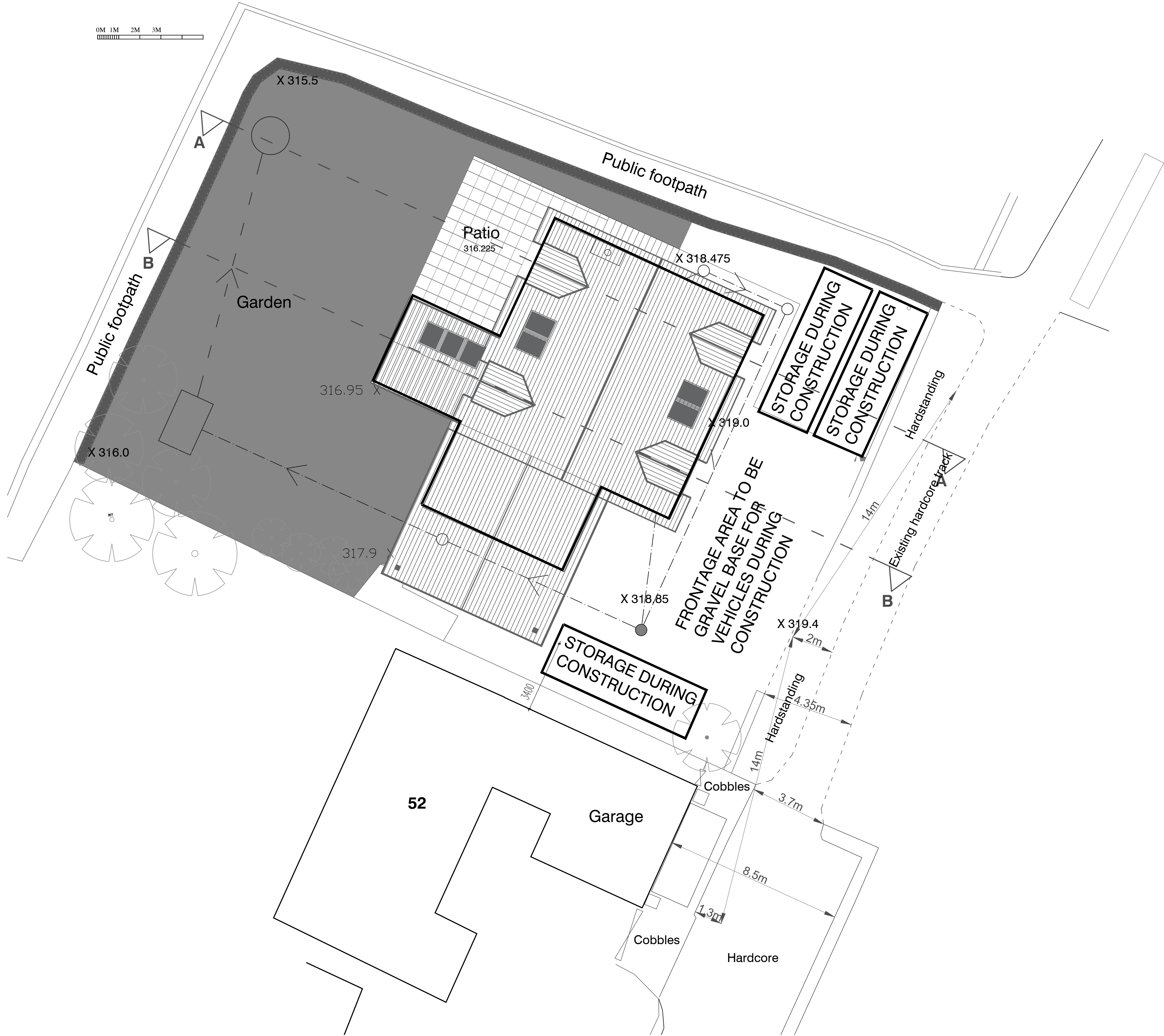
SITE STORAGE AND PARKING DURING CONSTRUCTION 1:100
