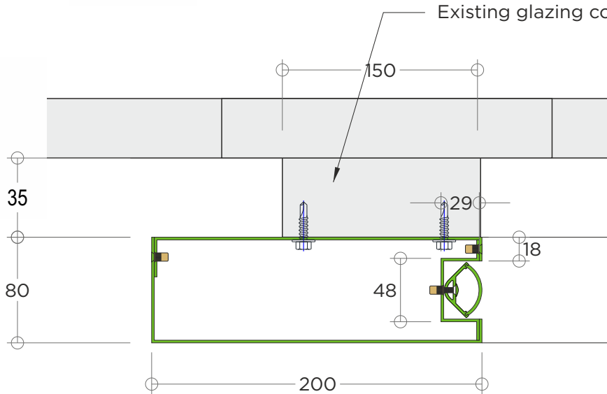
Left Section 1:4
