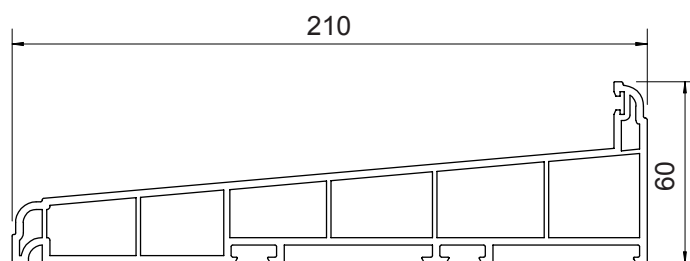
VS14 Extended Cill
