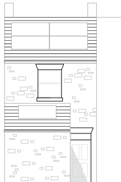
south west elevation — as proposed
