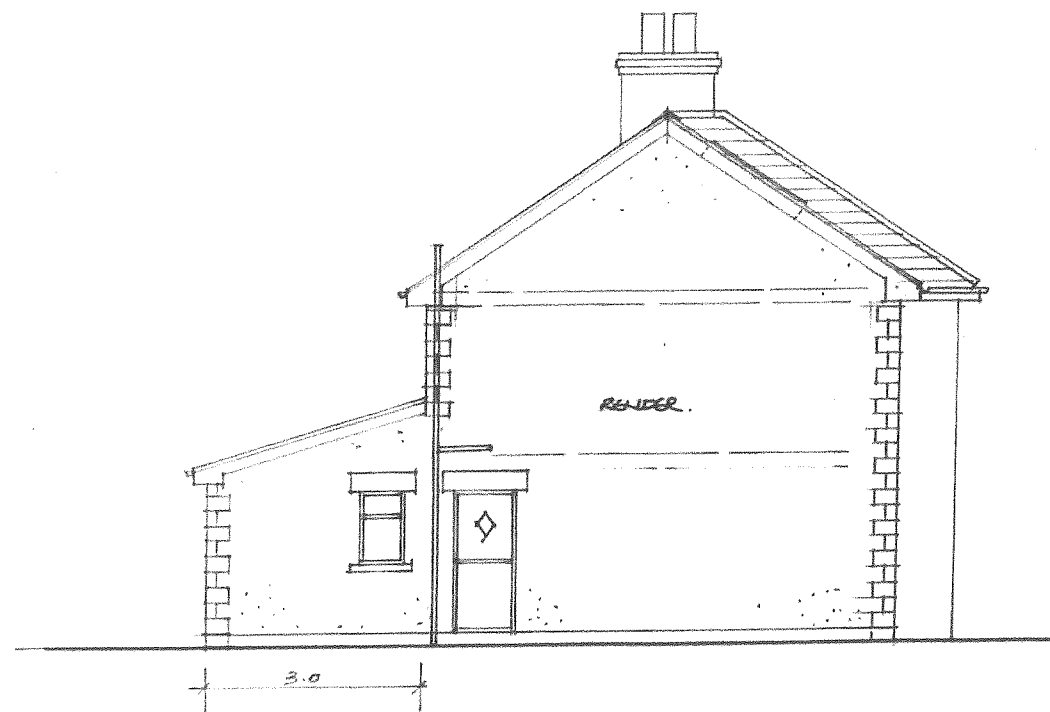
PROPOSED SIDE ELEVATION \ S.W.
