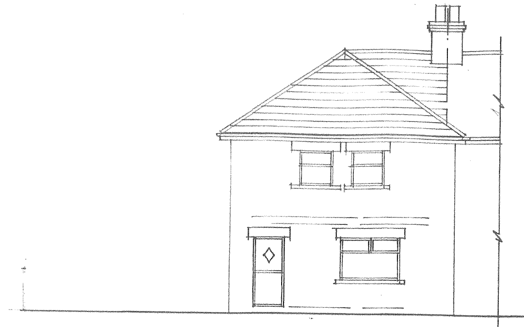
FRONT ELEVATION S.E.
