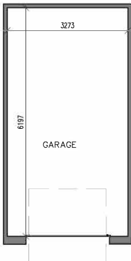
Ground Floor Plan 1:100 Total Floor Area 20.2m²
