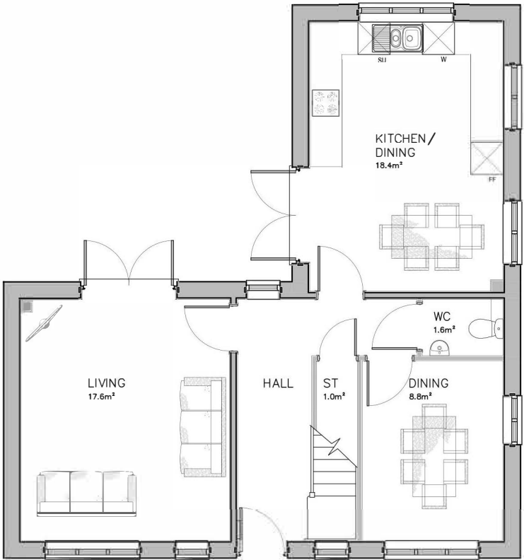
Ground Floor Plan 1:100 Total Floor Area 120.5m² Plots 1, 359, 381
