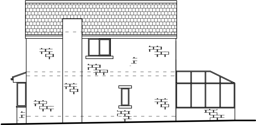
Side (South)
