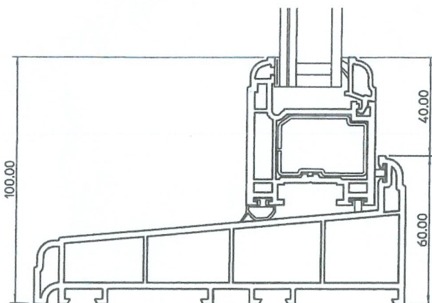
Bottom Rail
