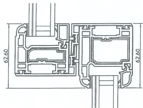
Meeting Rail
