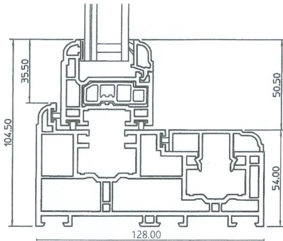
Top Rail
