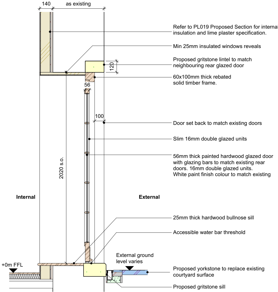
Window Section Detail Scale - 1:20
