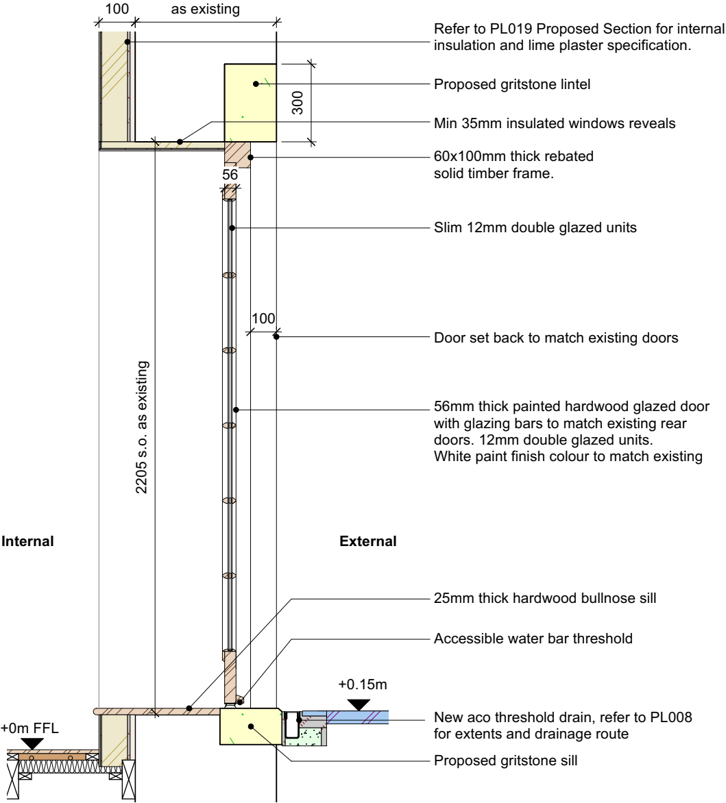
Window Section Detail Scale - 1:20
