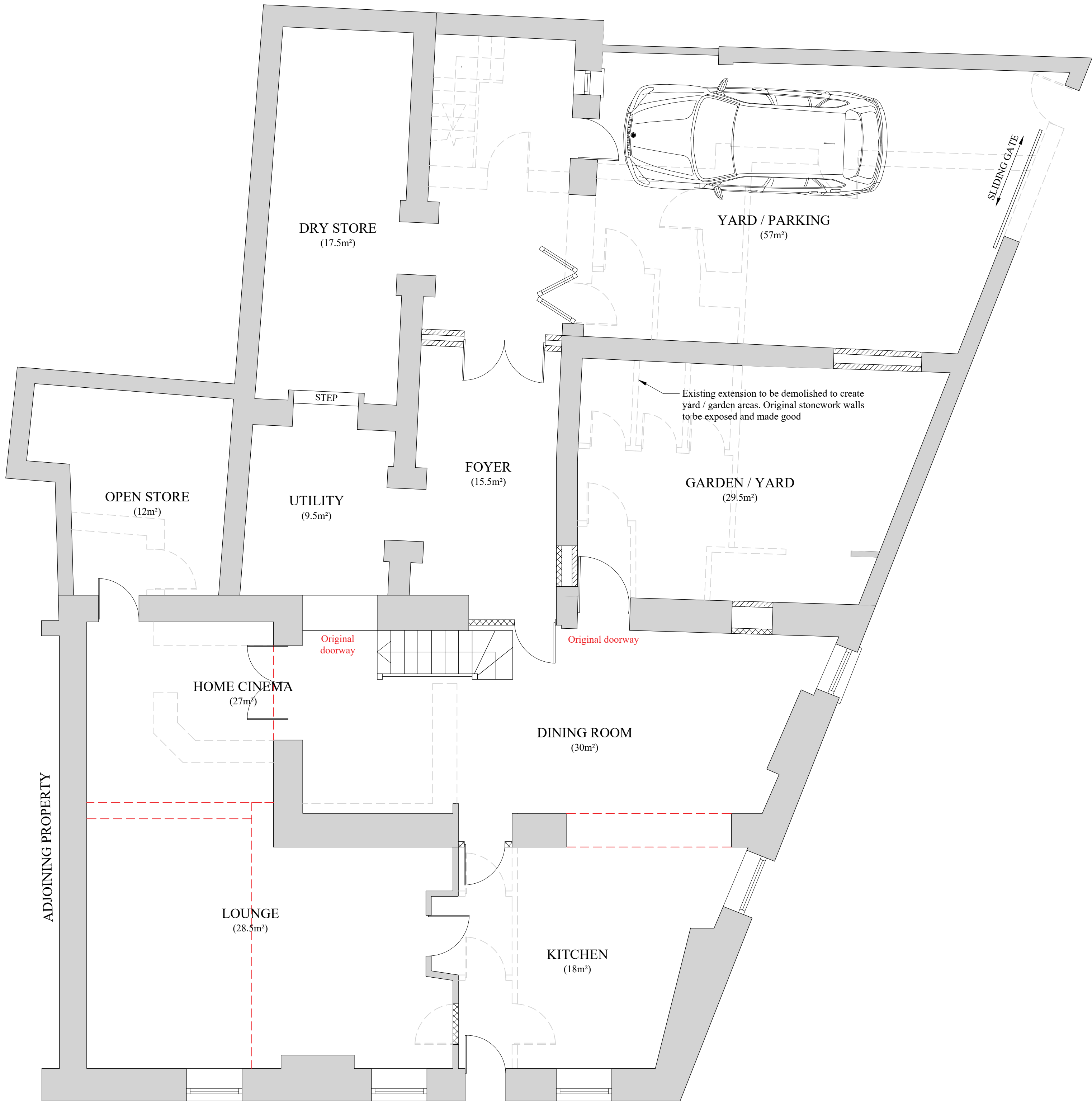
PROPOSED GROUND FLOOR LAYOUT (SCALE 1:50)
