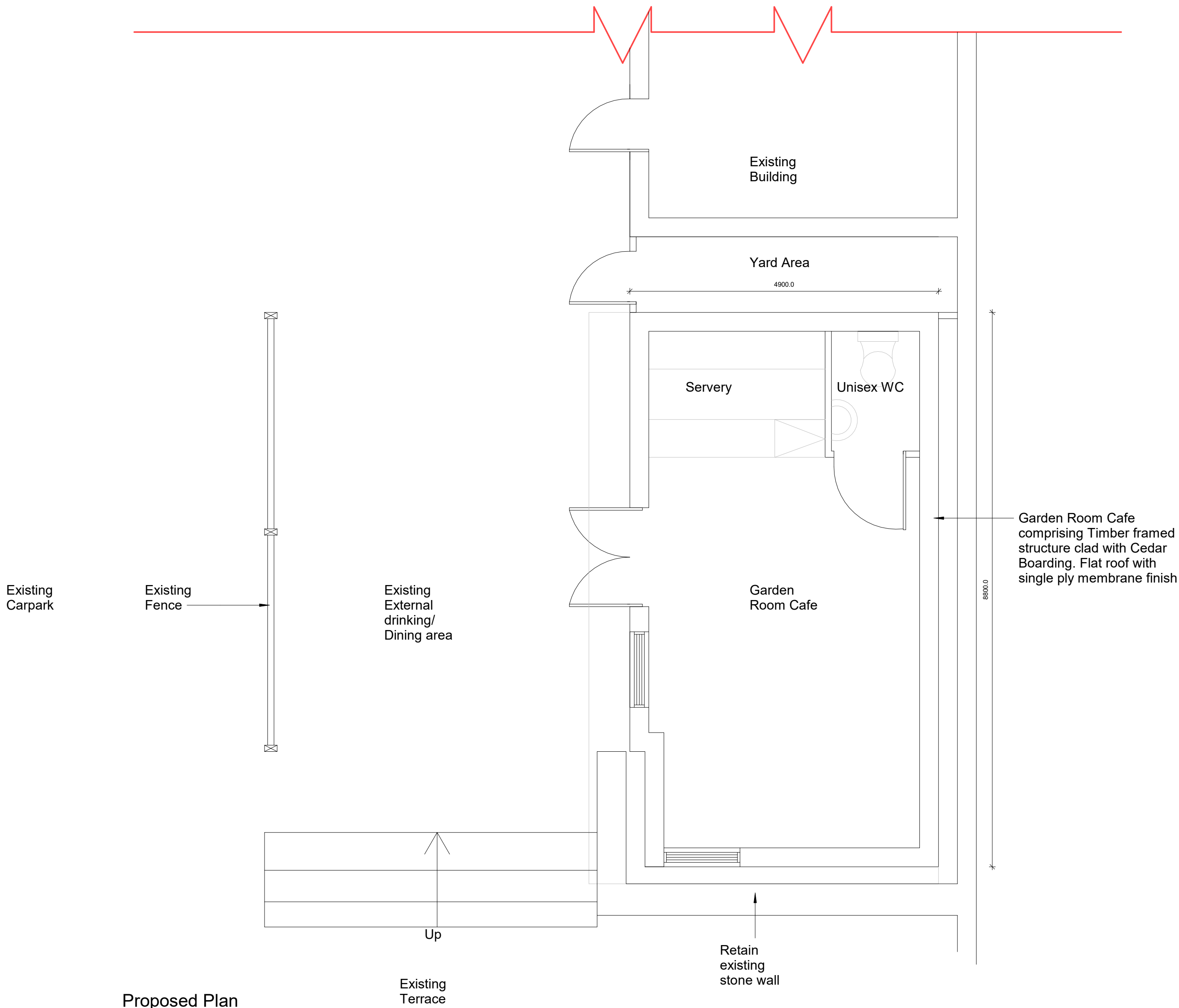
Proposed Plan 1 : 50
