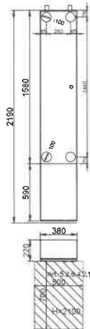
LANDING DOORS AND STRUCTURAL OPENING
