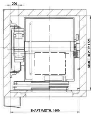
SECTION A-A CONTROL PANEL DIMENSIONS AND LOCATION
