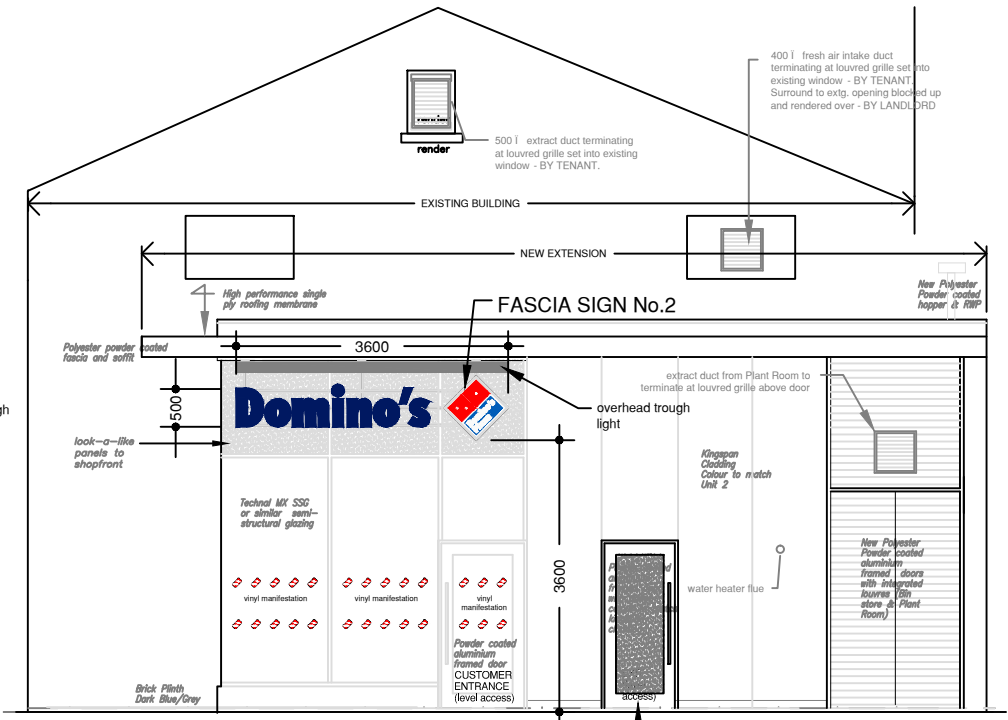
REAR (east) ELEVATION TO CAR PARK
