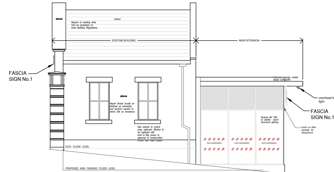
SIDE (south) ELEVATION TO ACCESS ROAD
