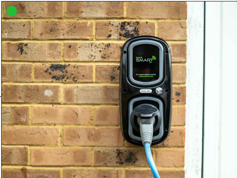
Example of wall mounted EV charging point - Mode 3.
