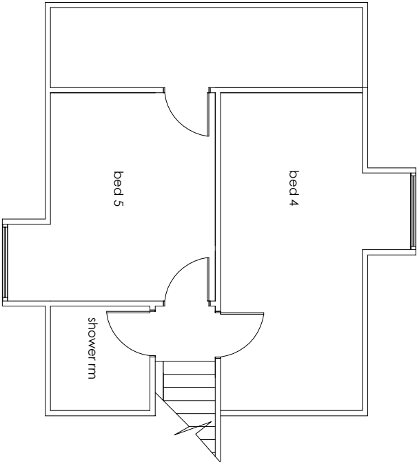
proposed second floor plan (as existing)
