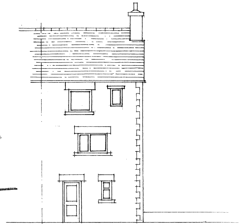
EAST ELEVATION 1:100
