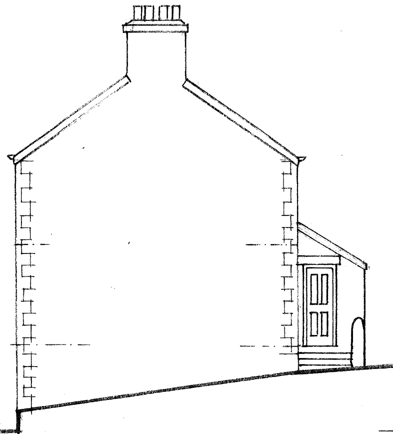
NORTH ELEVATION 1:100
