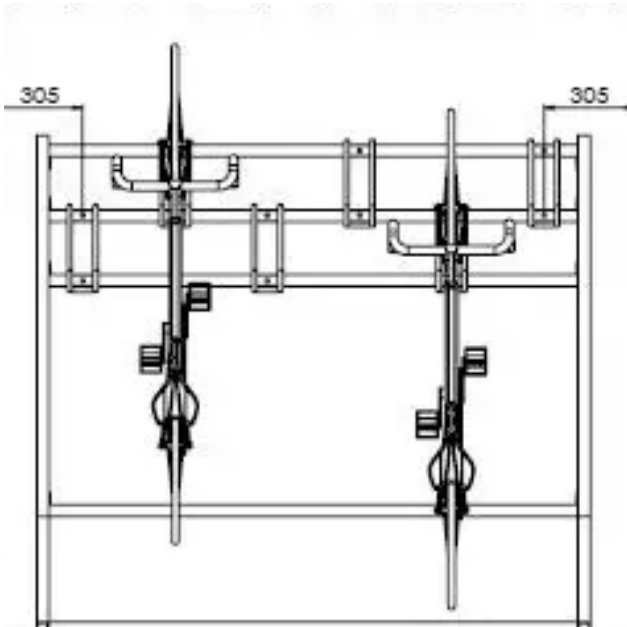
Plan view of vertical stacking mechanism
