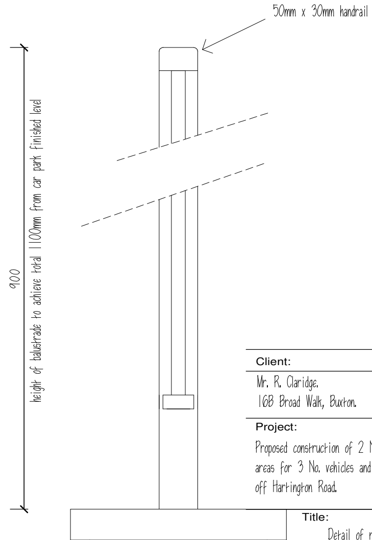
Cross section
