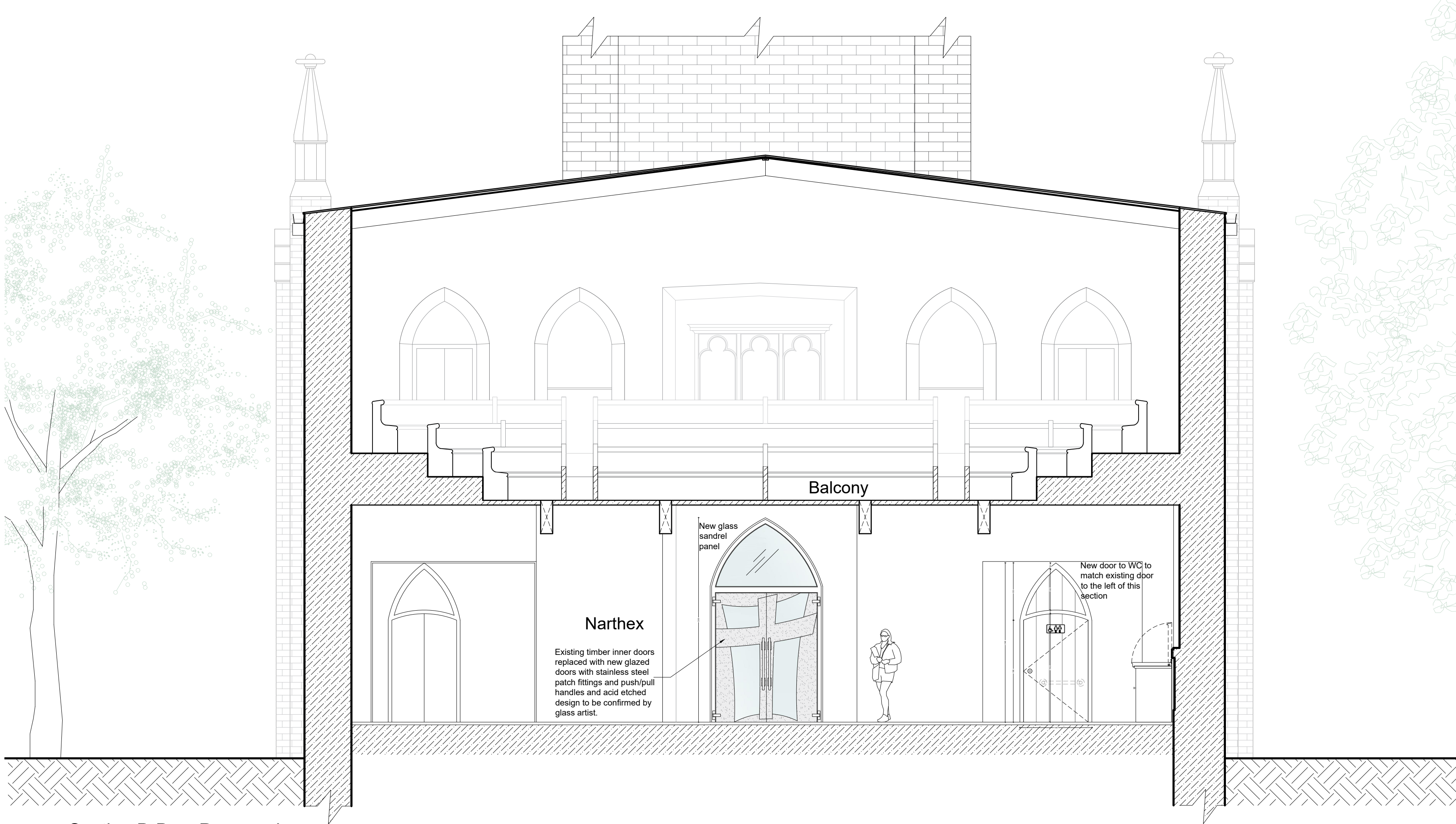
Section B-B as Proposed
