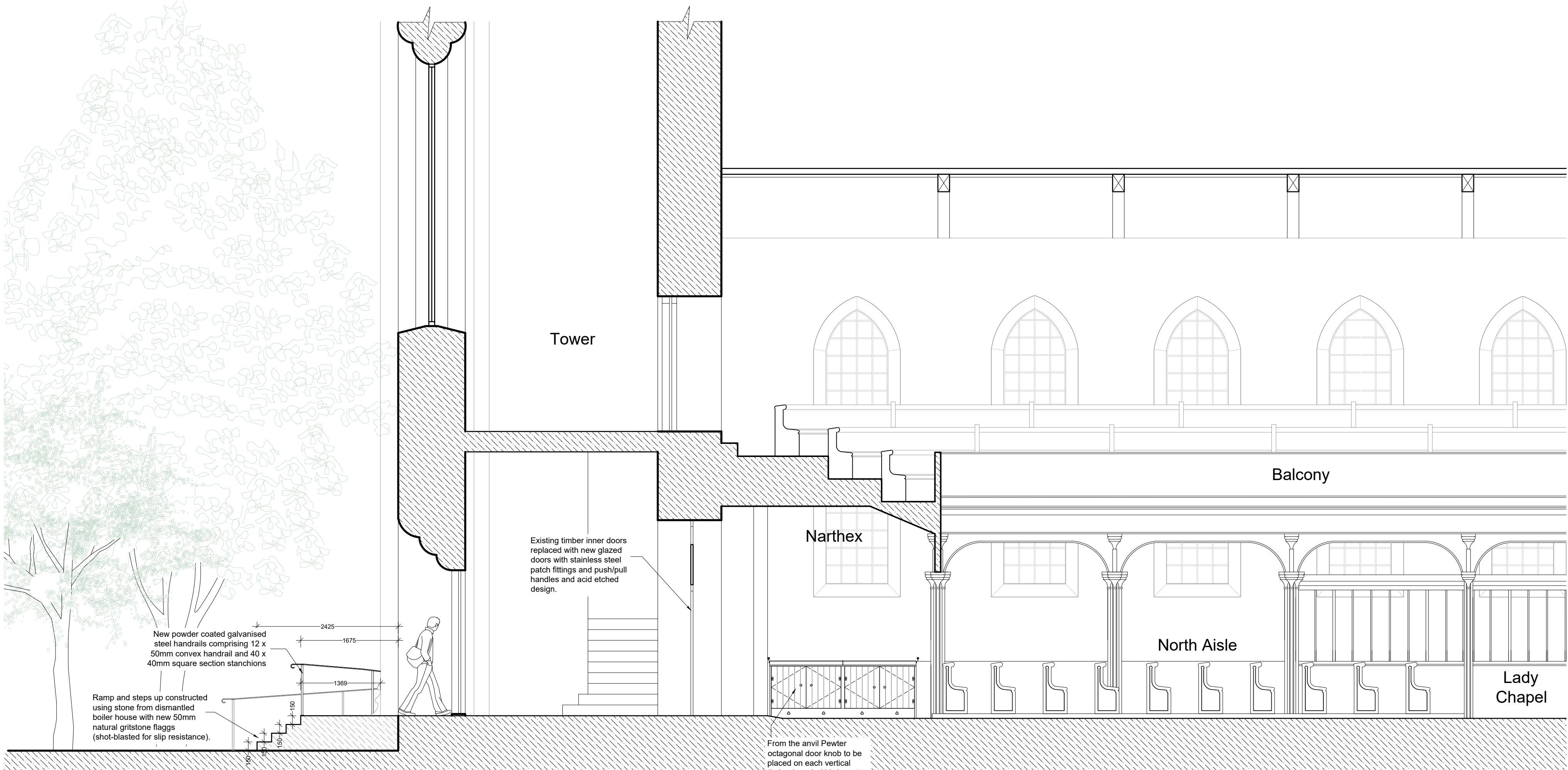
Section A-A as Proposed
