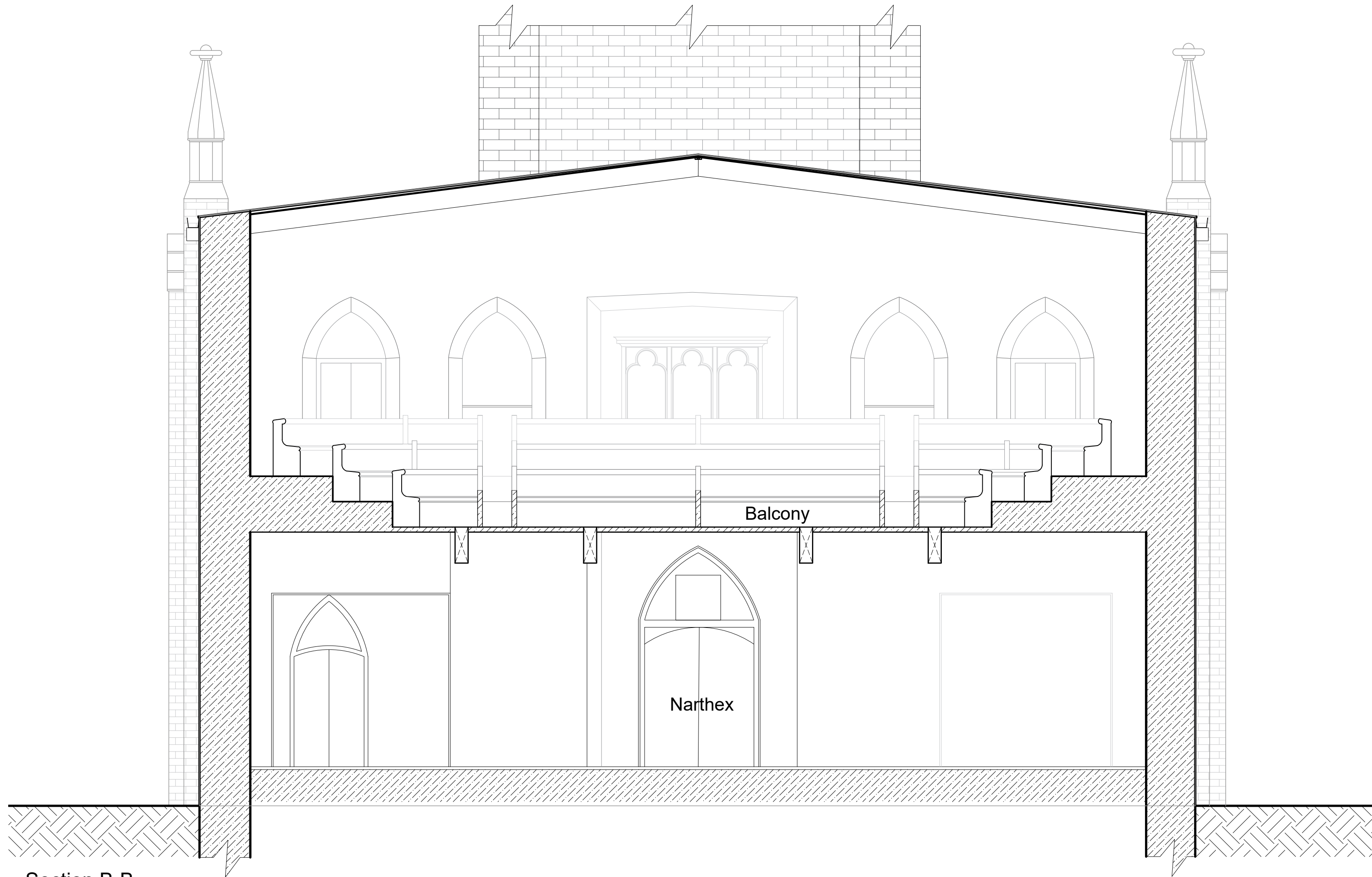
Section B-B (Scale 1:50)
