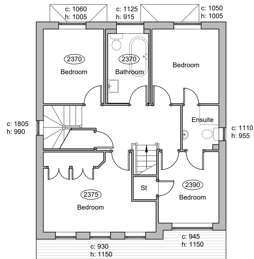
FIRST FLOOR - 1:100
