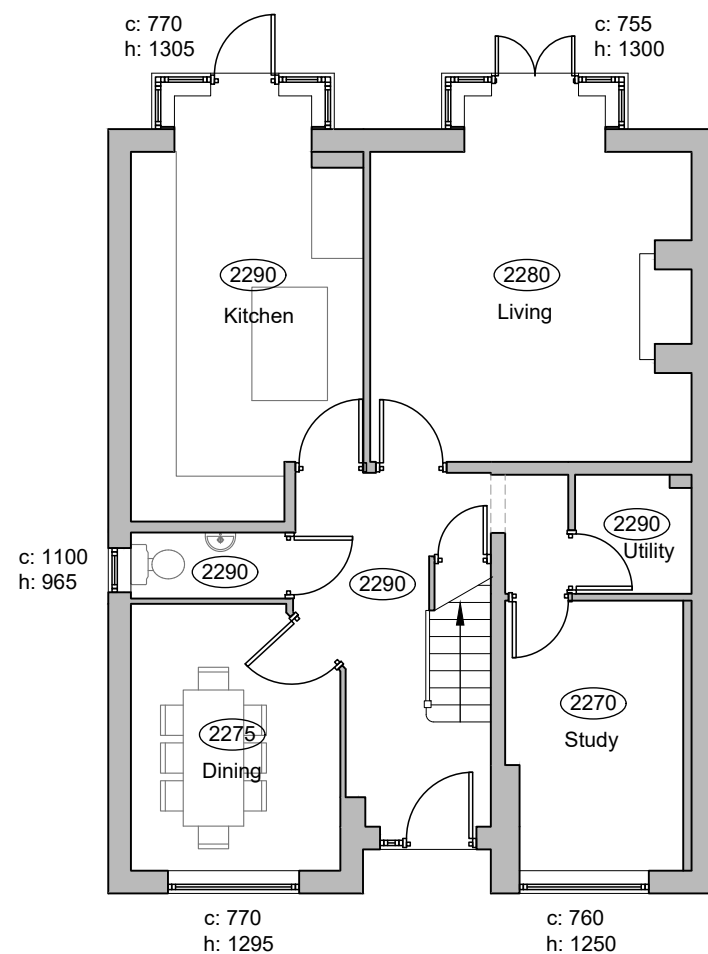
GROUND FLOOR - 1:100
