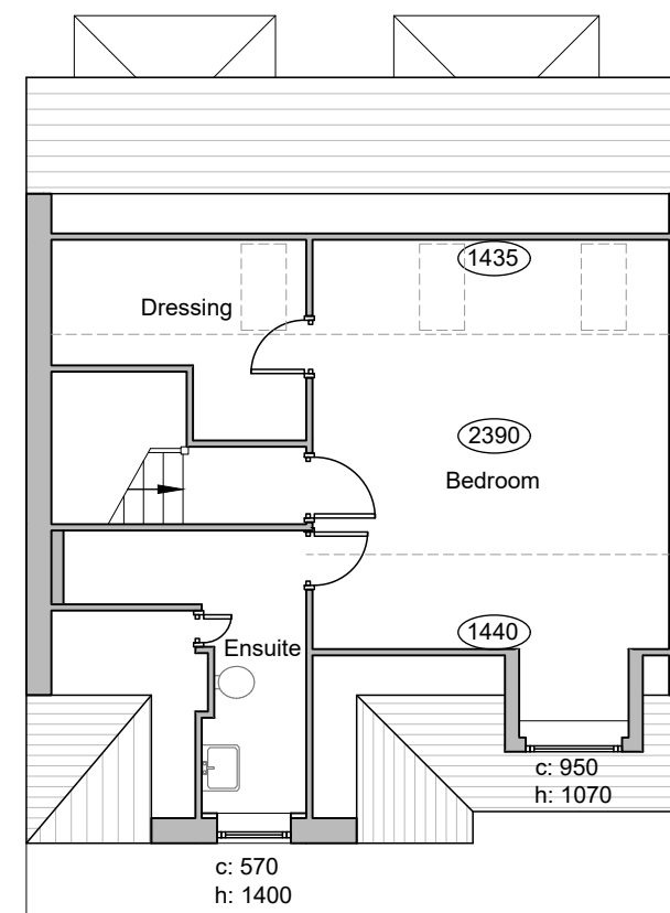
SECOND FLOOR - 1:100
