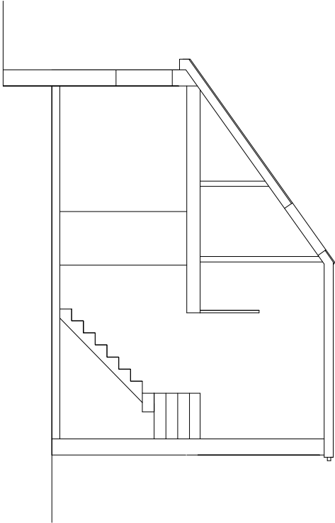
proposed section A-A
