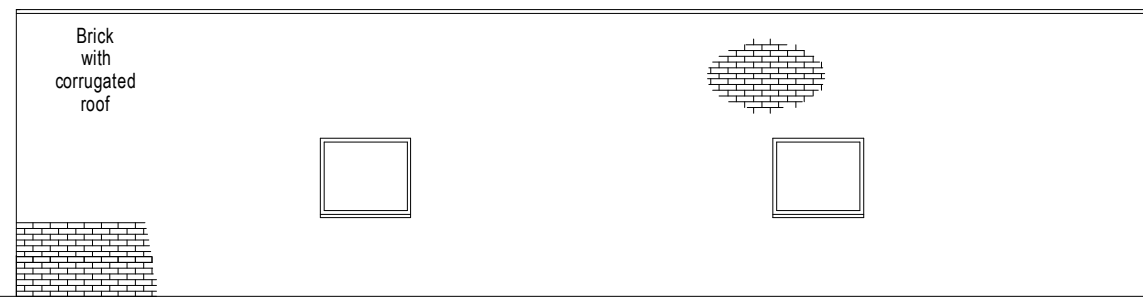
NW Elevation
