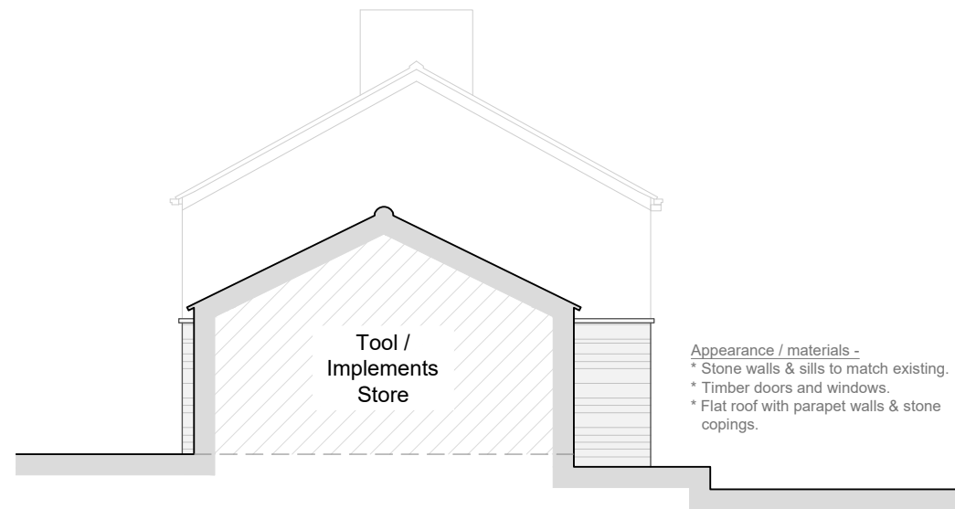
Side / East elevation
