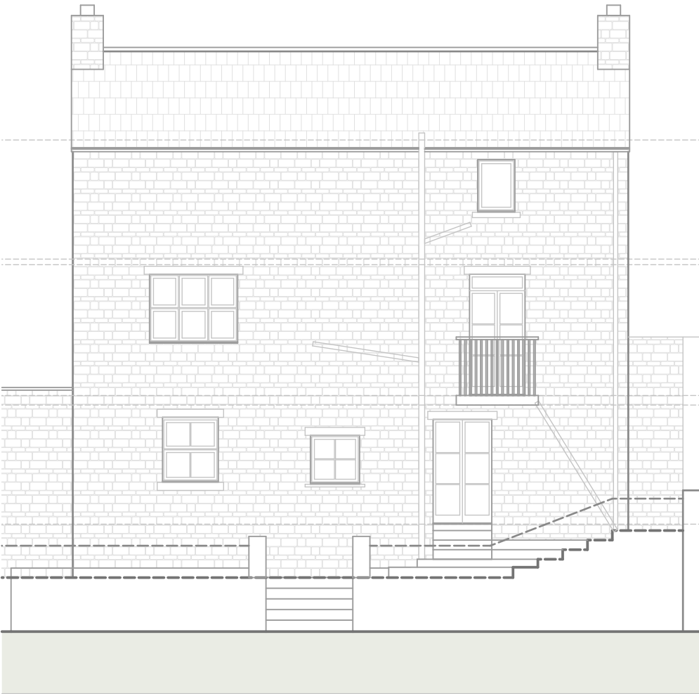
West Elevation
