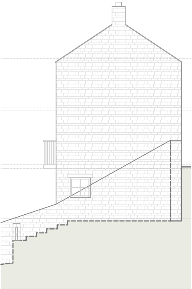
South Elevation
