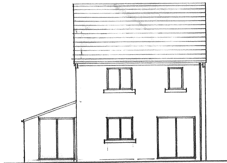
REAR ELEVATION EAST
