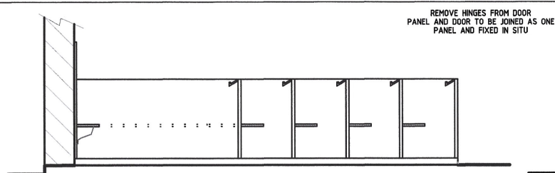
PROPOSED SECTION A-A
