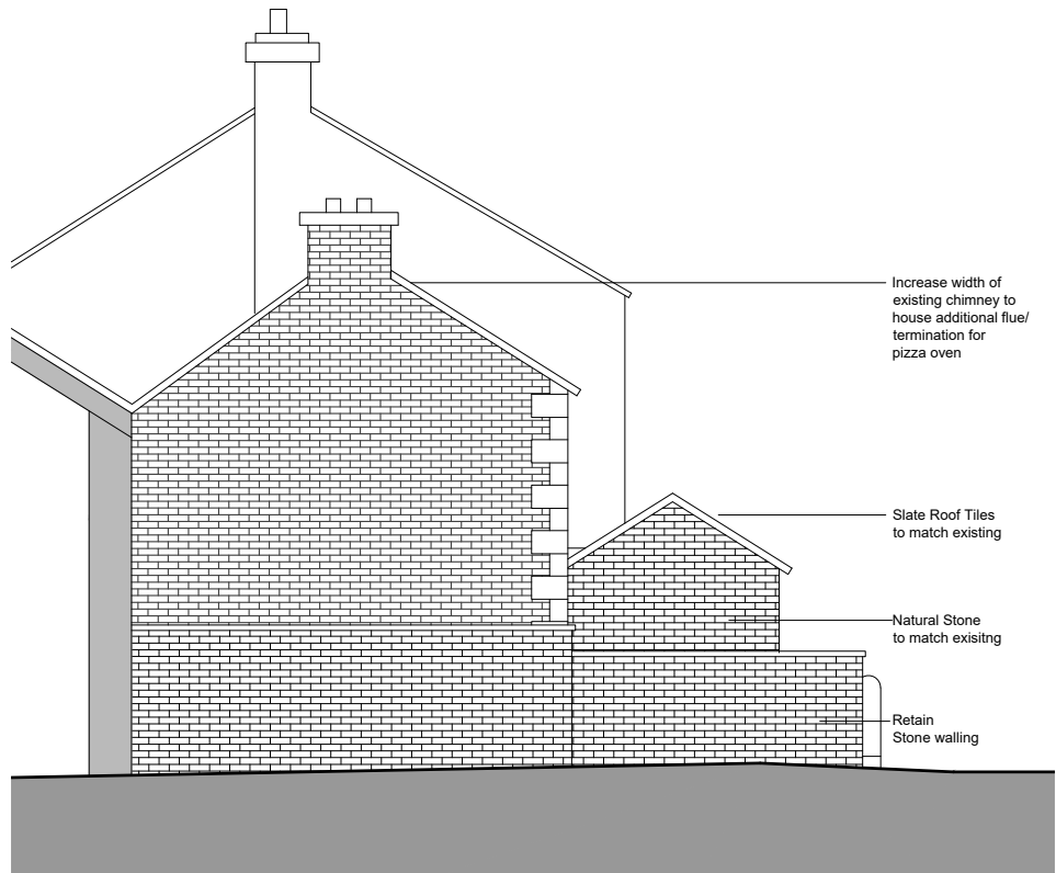
North Elevation (side) 1:100
