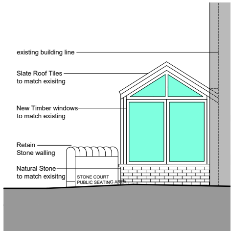
South Elevation (side) 1:100
