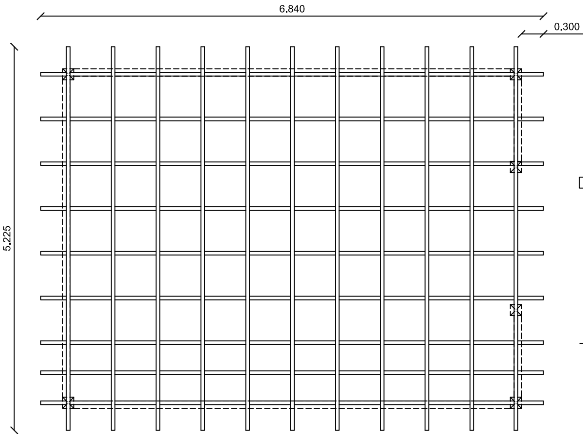
Roof Plan
