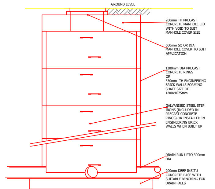
TYPICAL MANHOLE DETAIL FOR INVERT LEVELS >1.0m <3.0m DP
