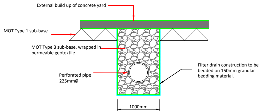
TYPICAL LAND DRAIN DETAIL
