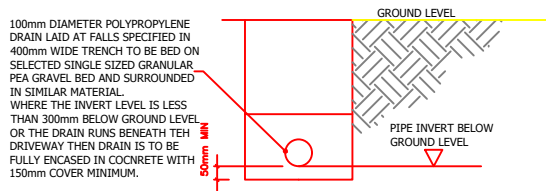
TYPICAL PIPE BEDDING DETAIL
