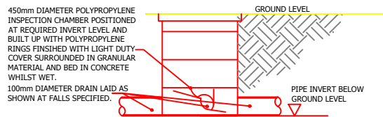
TYPICAL INSPECTION CHAMBER DETAIL FOR INVERT LEVELS <1.0m DP
