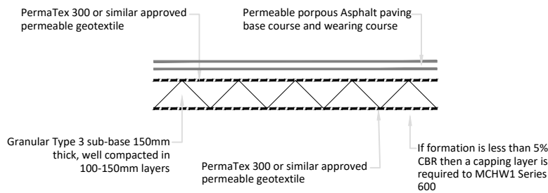
CAR PARK CONSTRUCTION DETAIL
