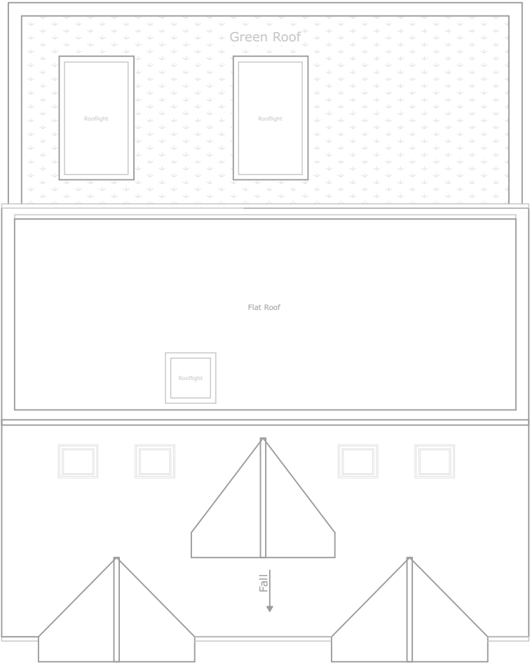
Roof Plan
