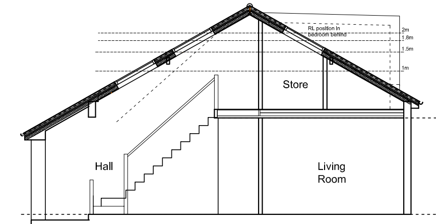
Sketch section at new entrance
