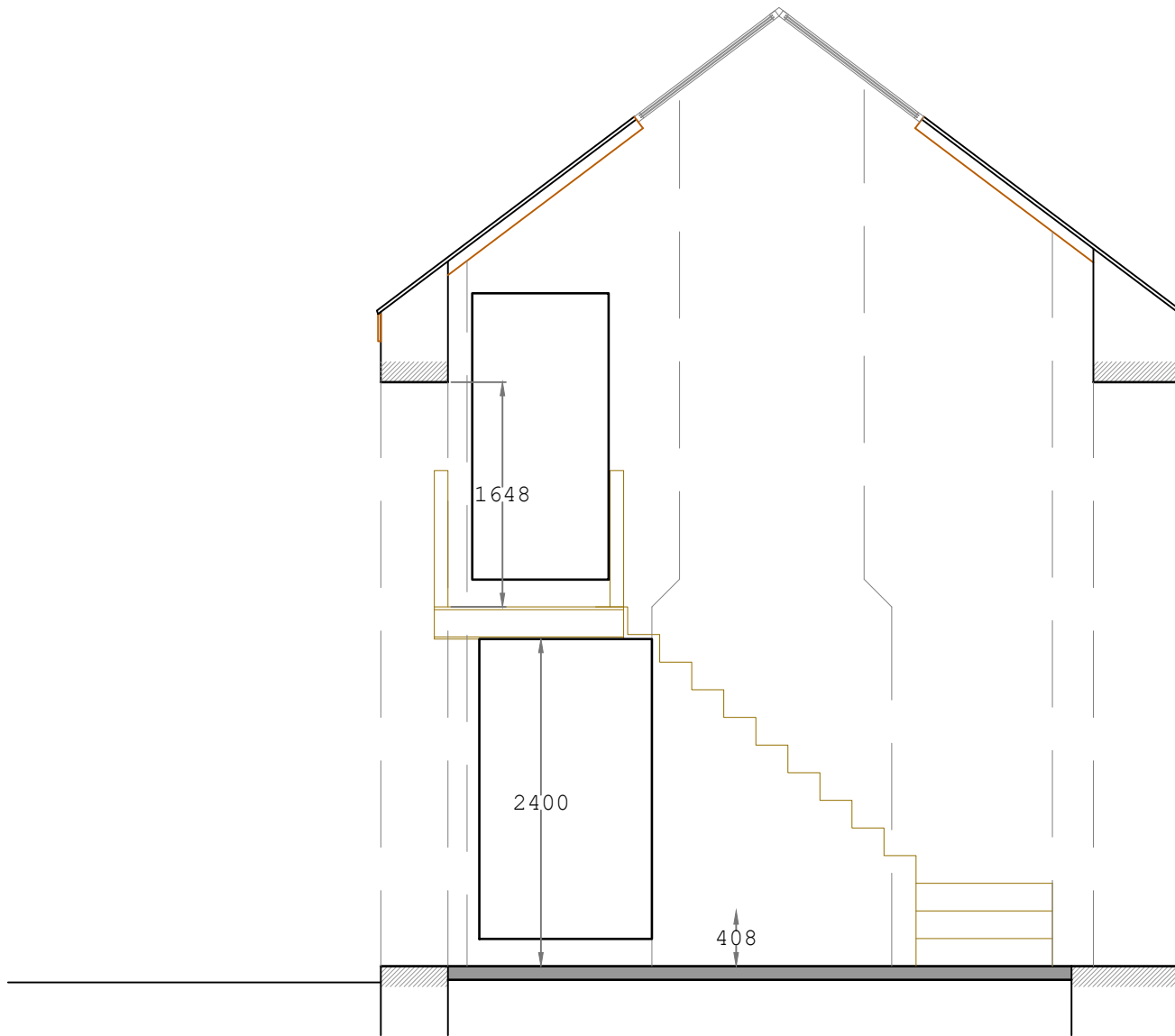
PROPOSED SECTION D-D
