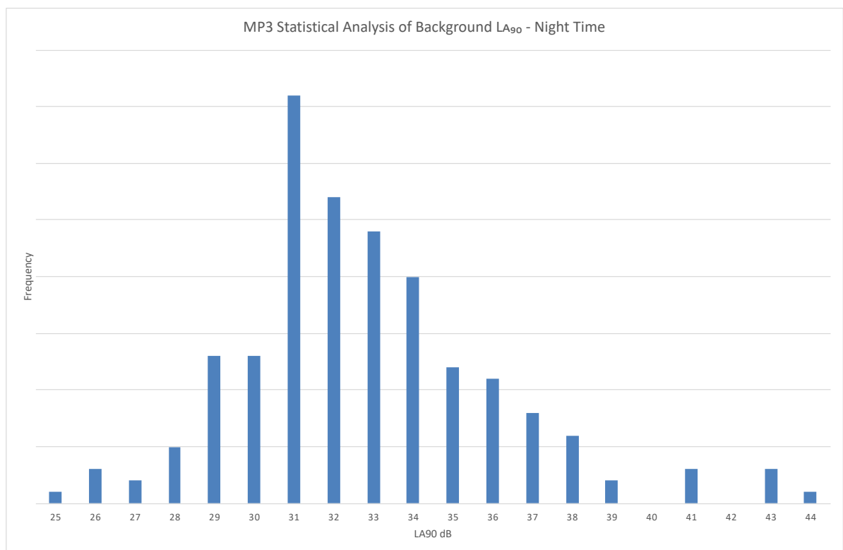
FIGURE 15: STATISTICAL ANALYSIS OF L_{A90} BACKGROUND – NIGHT-TIME – MP3
