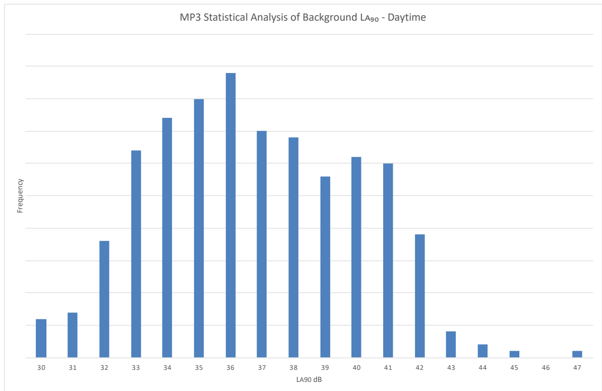
FIGURE 14: STATISTICAL ANALYSIS OF L_{A90} BACKGROUND – DAYTIME – MP3
