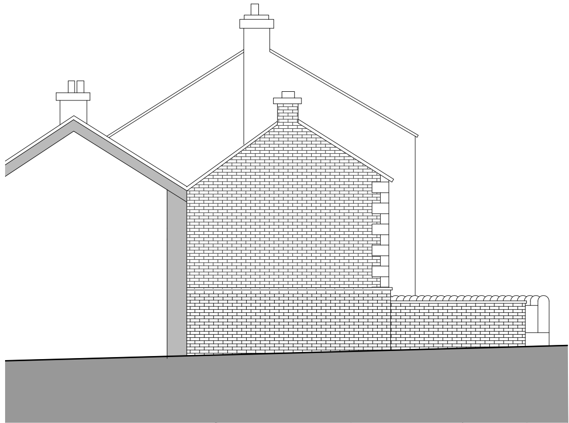
North Elevation (side) 1:100
