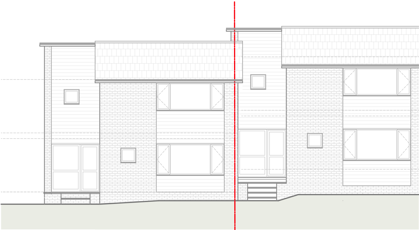
West Elevation
