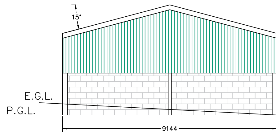
Southeast Gable Elevation
