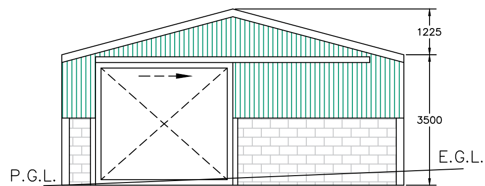
Northwest Gable Elevation
