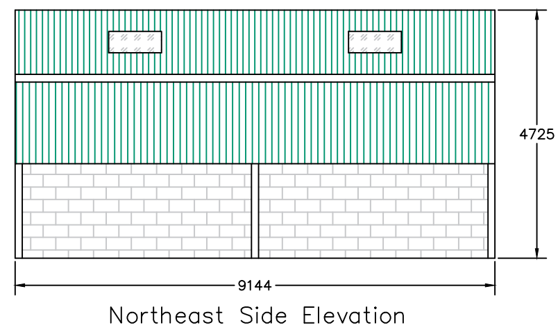
Northeast Side Elevation
