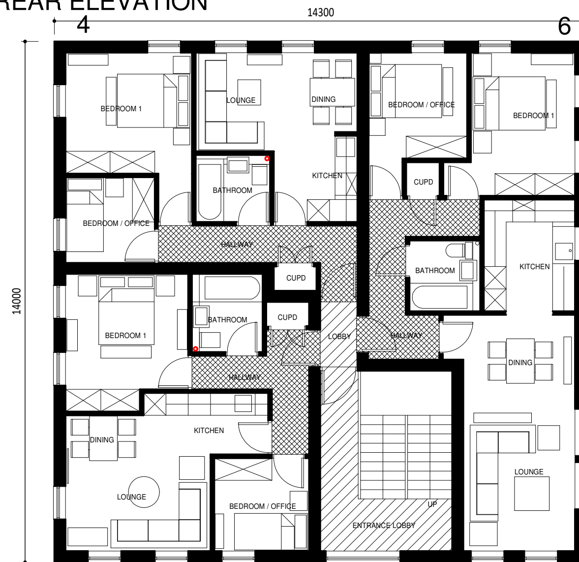
5 FIRST FLOOR PLAN
