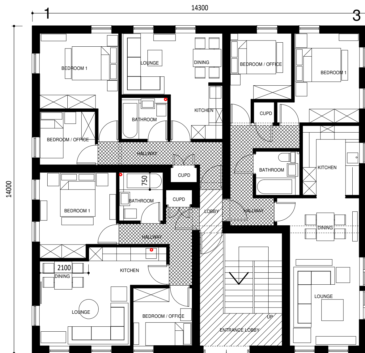
2 GROUND FLOOR PLAN
