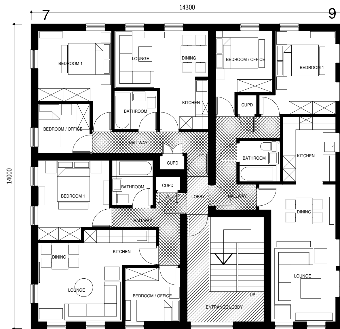
8 SECOND FLOOR PLAN
