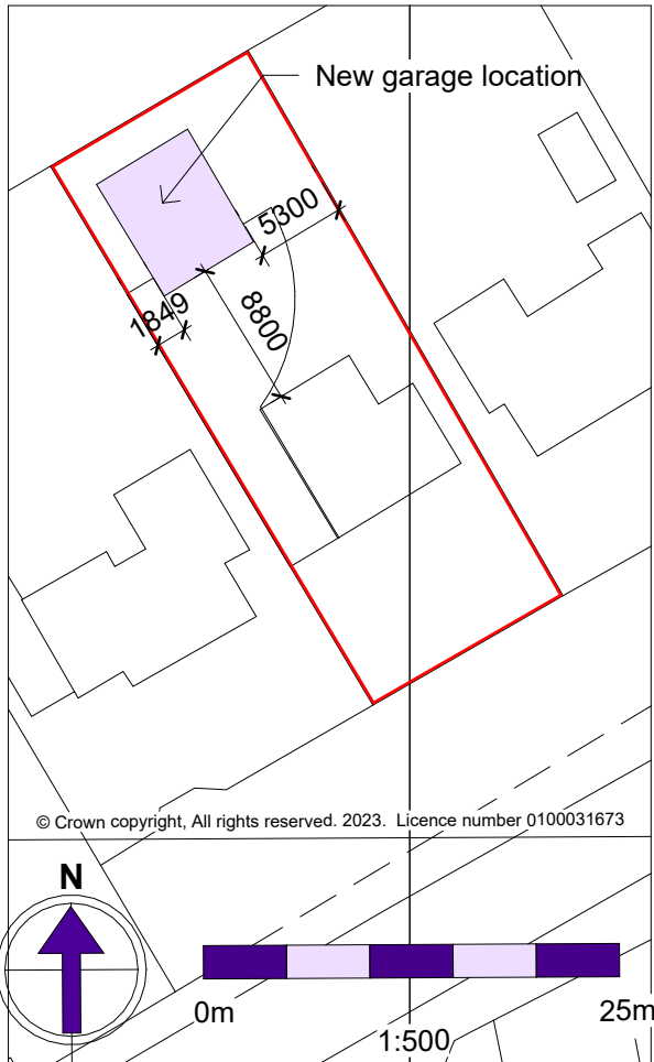
Site Plan - Proposed 1 : 500
