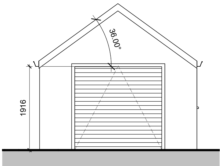
South Existing 1 : 50
