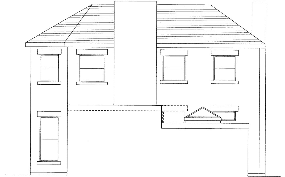
ELEVATION TO MANCHESTER ROAD
