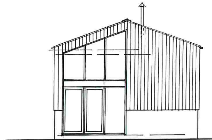
EAST ELEVATION.
