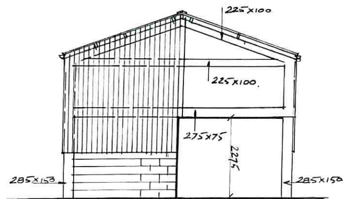
WEST ELEVATION
