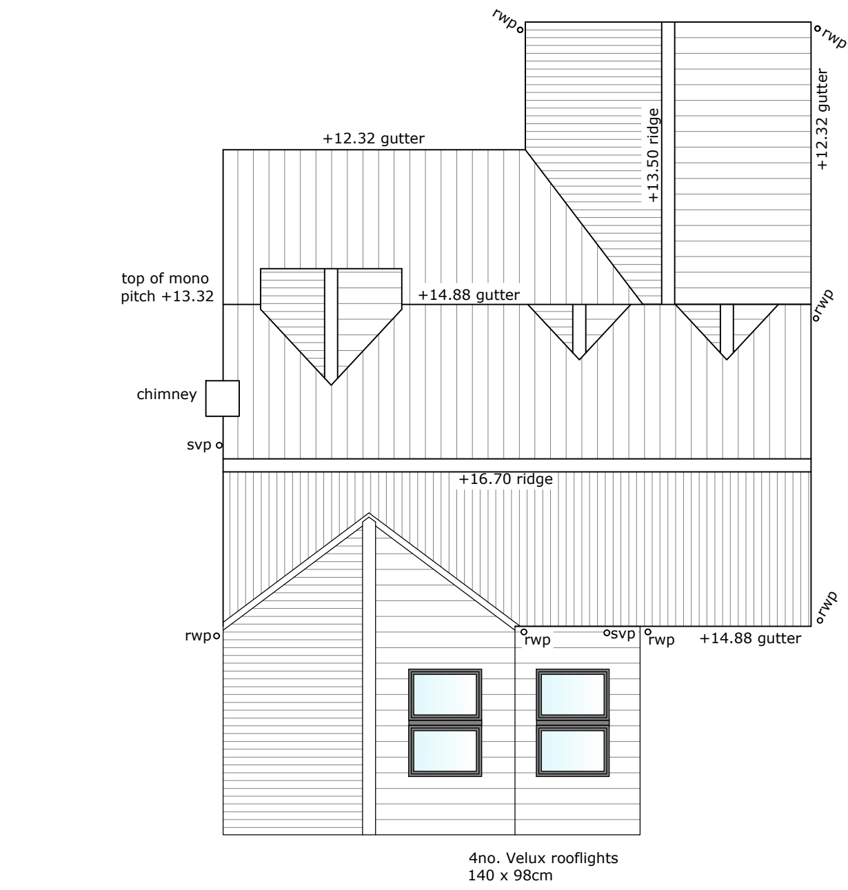
ROOF PLAN
