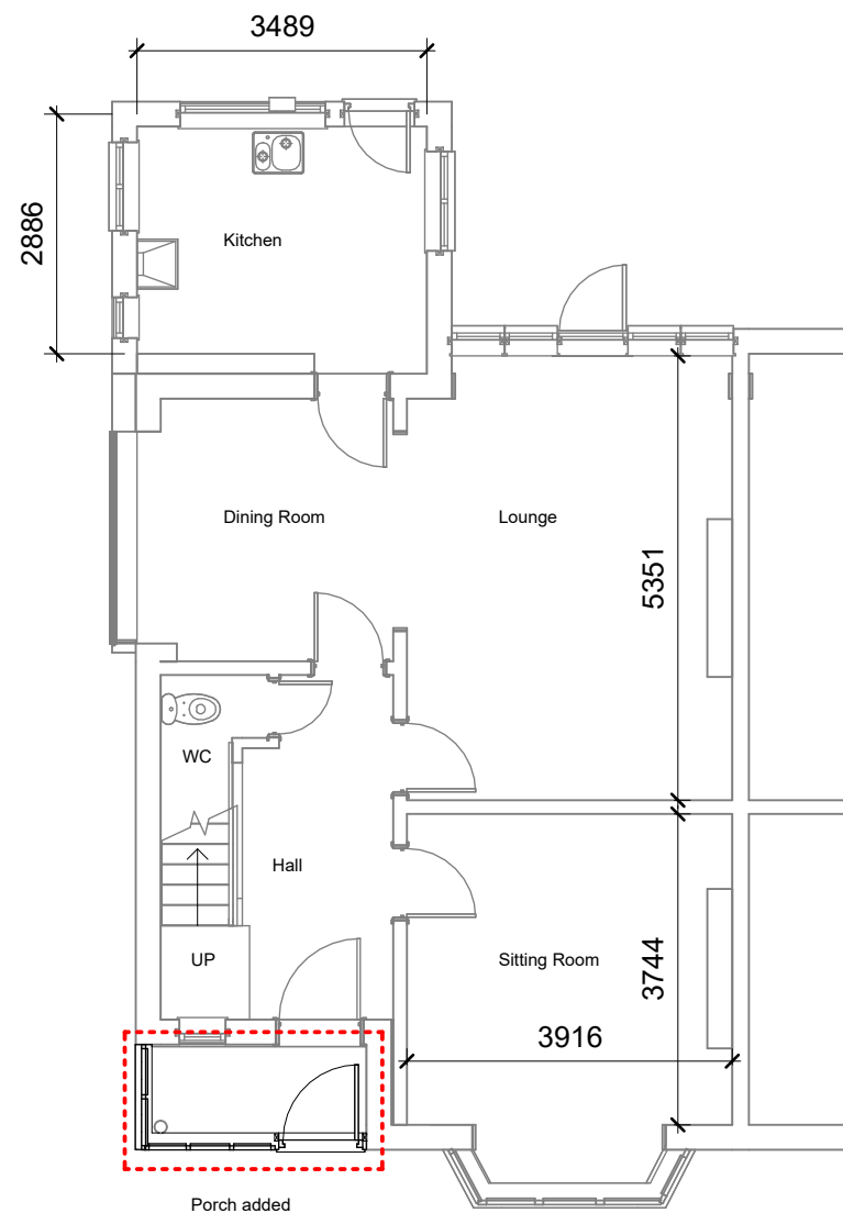
Ground Floor - proposed 1 : 100
