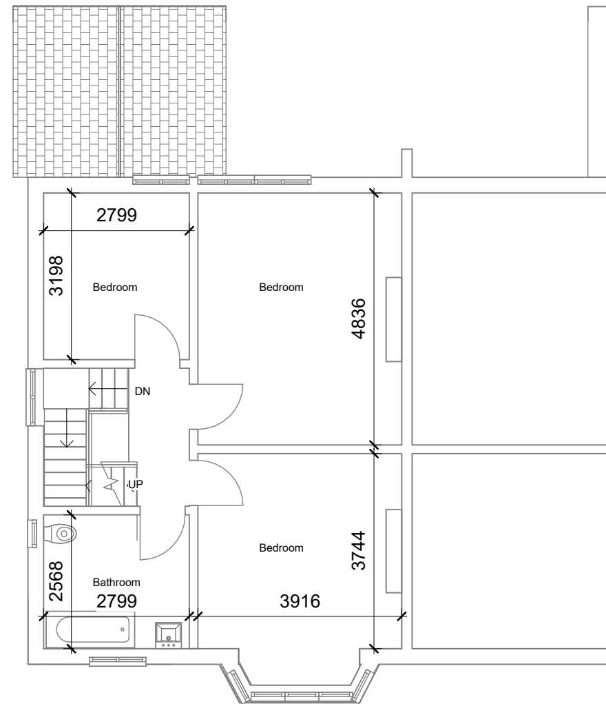
First floor- proposed 1 : 100
