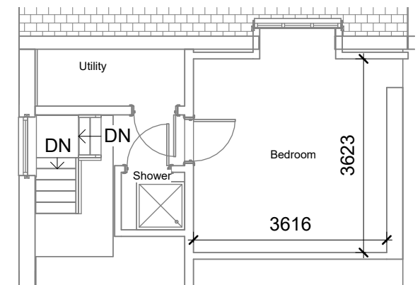
Second floor - proposed 1 : 100
