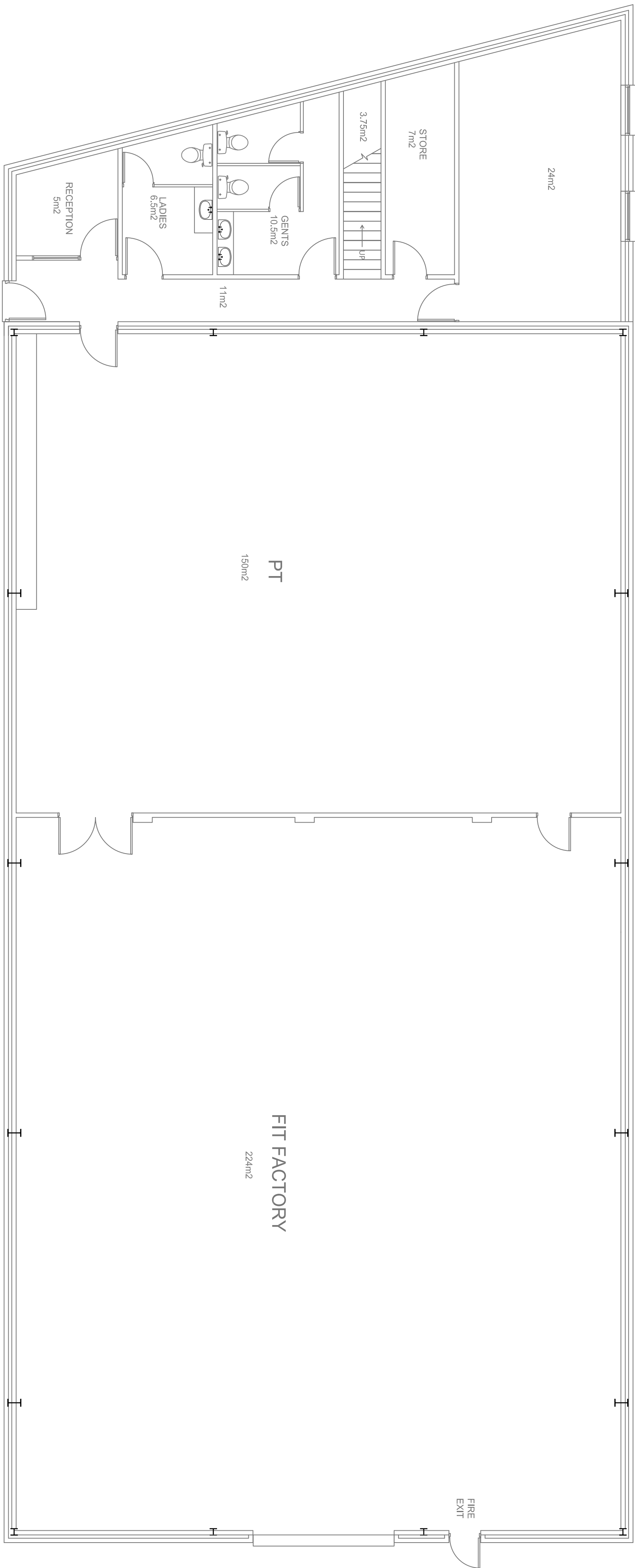
GROUND FLOOR PLAN - 1:100
